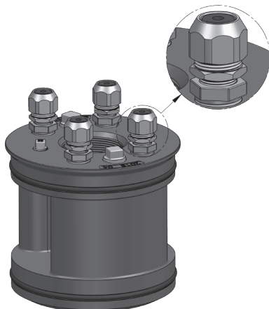
Flowing well spool for 10" Ductile Iron Pitless Unit. Currently only available with 6" FPT drop pipe connection.
