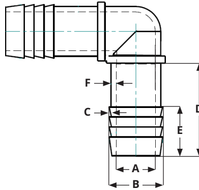
PVCE Series - Insert Elbow
