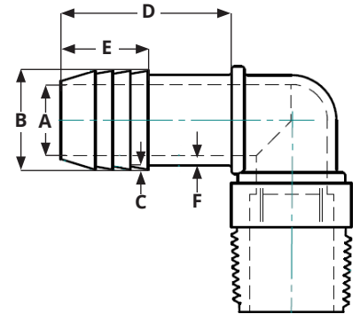
PPME Series - Male Insert Elbow
