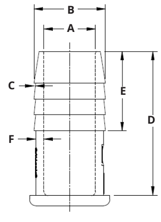
PVCP Series - Plug Adapter
