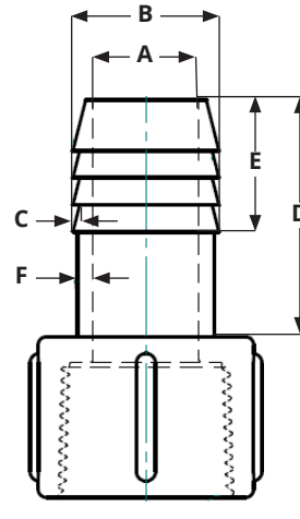
PVCFA Series - Female Insert Adapter
