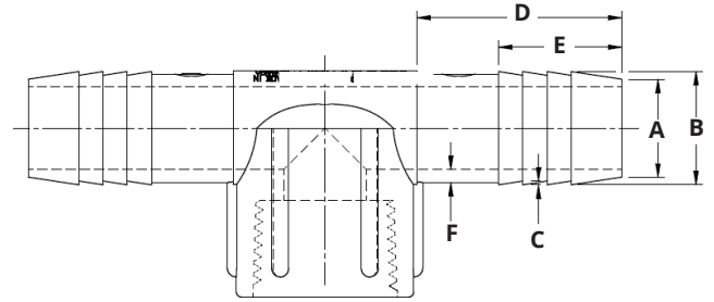
PVCFT Series - Female Insert Tee
