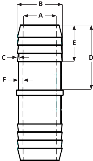
PVCC Series - Insert Coupling
