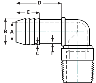
NME Series - Male Insert Elbow
