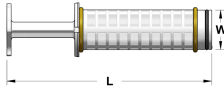
Separator Element
